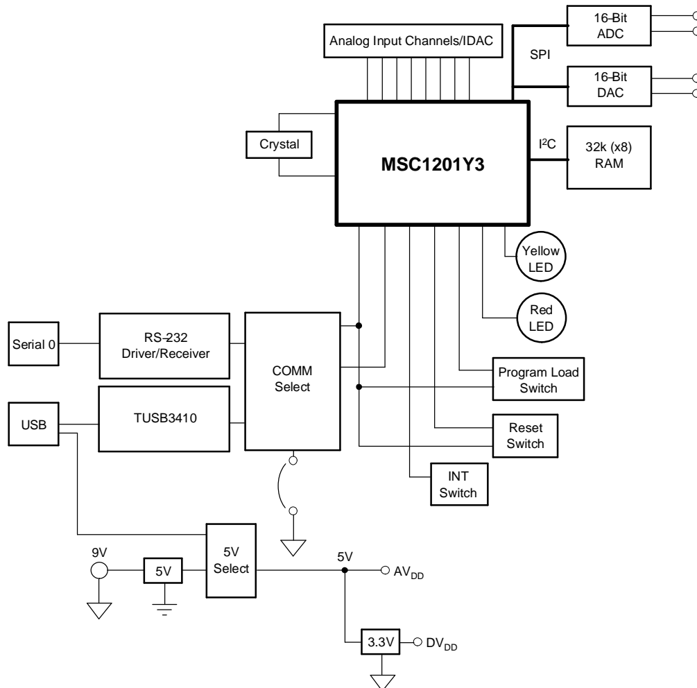
Figure 1. MSC1201/02EVM Overview
